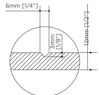
V-GROOVE DETAIL VIEW
